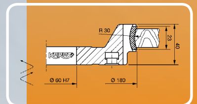
Diamond High Speed Profile Cutters with Quick Release System
