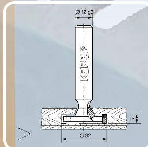
CNC Diamond T-Slot Routers
