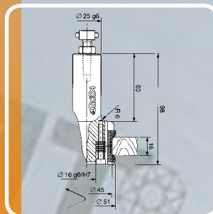
CNC Diamond Adjustable Routers
