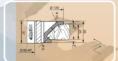
Diamond Cutters for Furniture Industry
