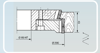
Diamond Cutters for Dooring Industry
