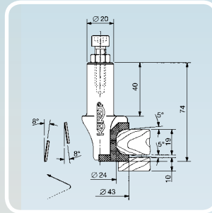
CNC Diamond Profile Routers
